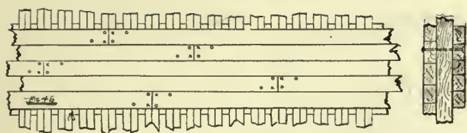
Fig. 46. Butt Fastenings
