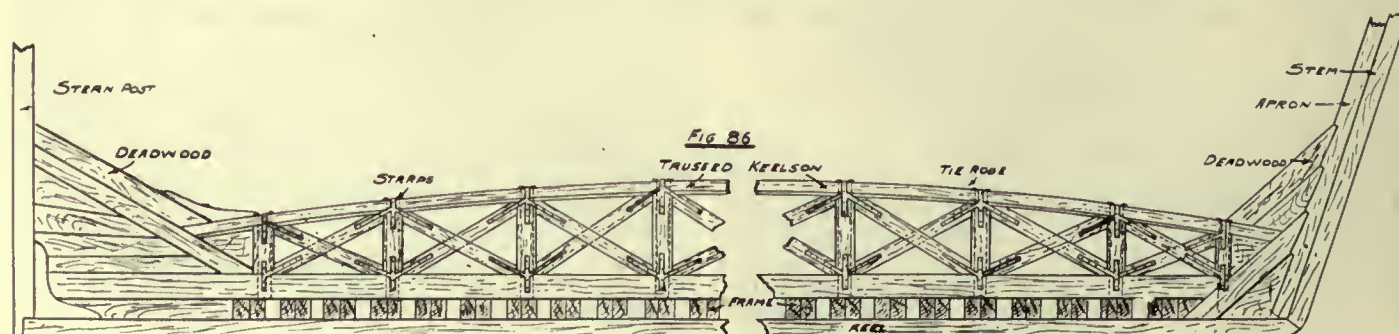
Fig. 88. Trussed Wood Keelson
