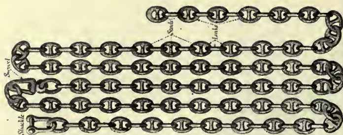
Fig. 165. Anchor Chain
