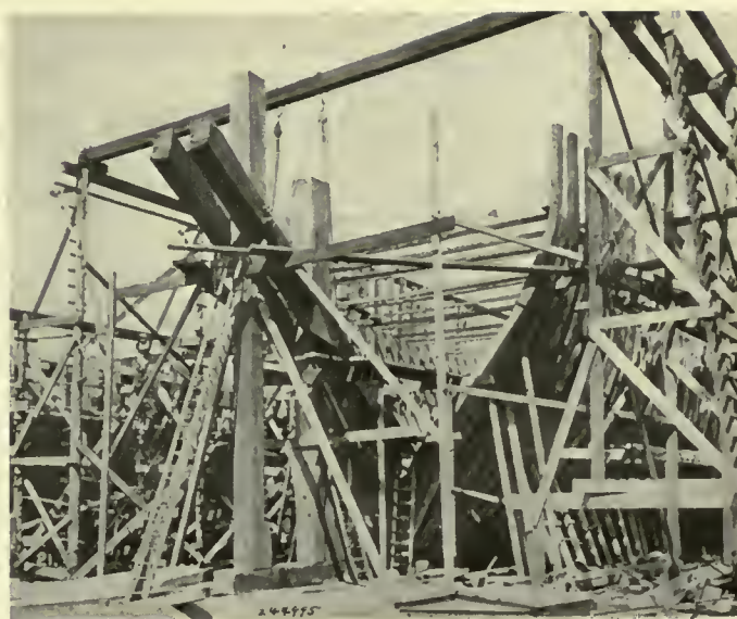
Fig. 38. Side Counter Timbers
