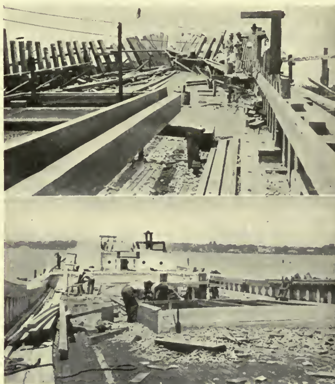
Fig. 96. View of Main Deck, No. 1 Hatch From Forward House Looking Aft
