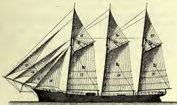
Fig. 108. Fore-and-Aft Schooner
