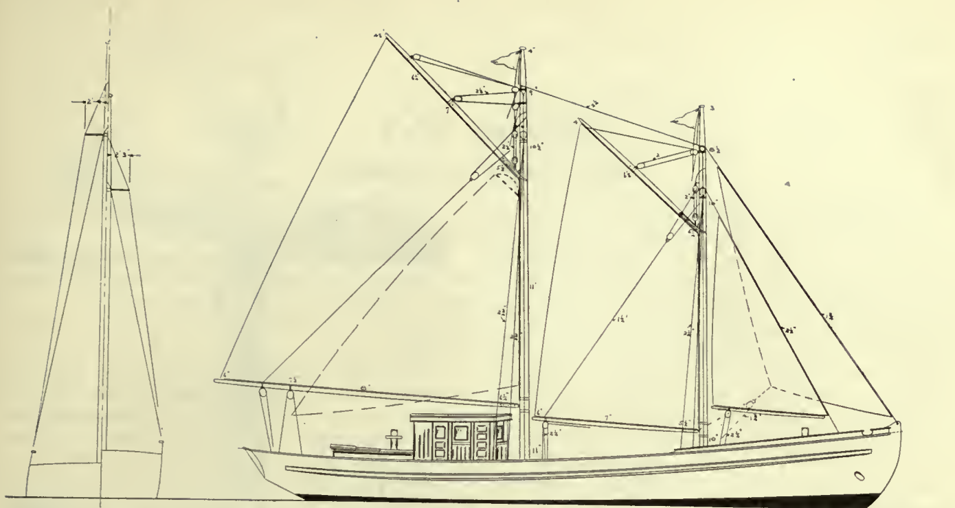
Fig. 151. Iskum, an 80-Foot Fishing Schooner Built From Designa by Edson B. Schock and Fitted With a Corliss Gas Engine
