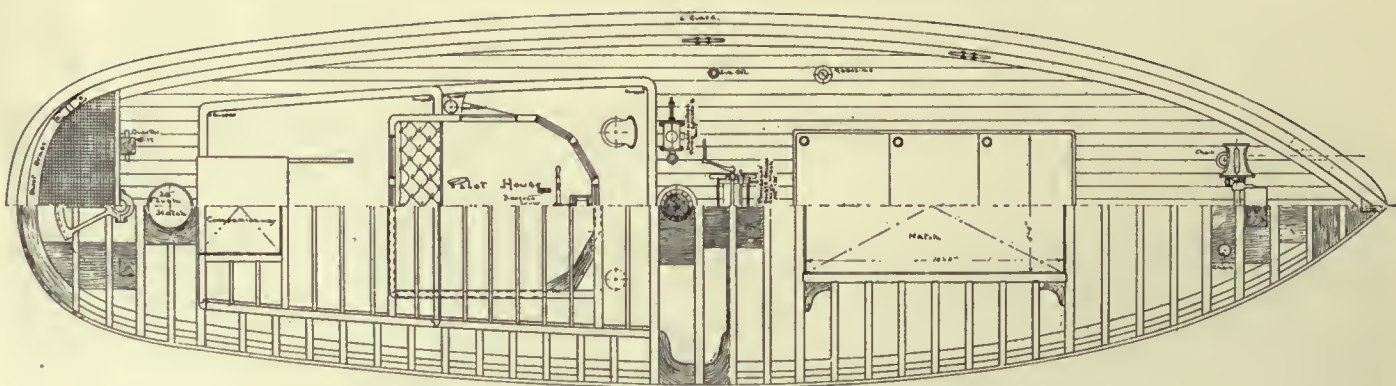
Fig. 146a. 52-Foot Hydro-Aeroplane Tender, Designed by J. Murray Watts
