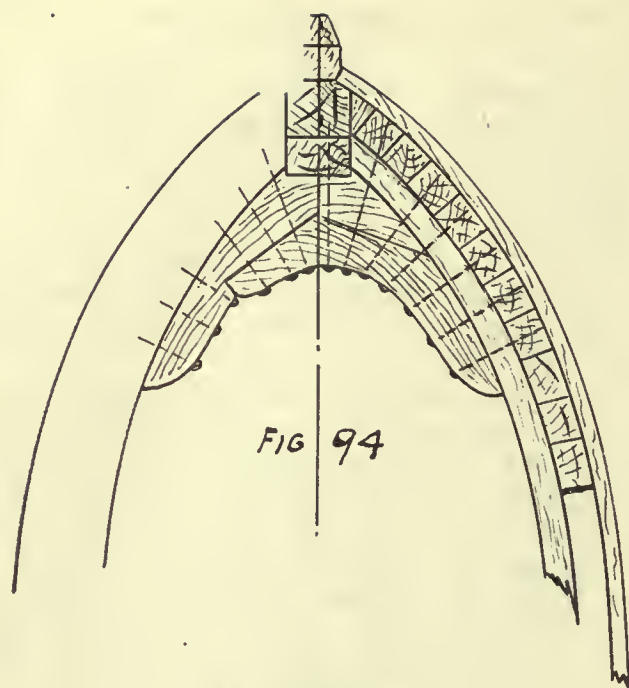
Fig. 94. Breast Hook
