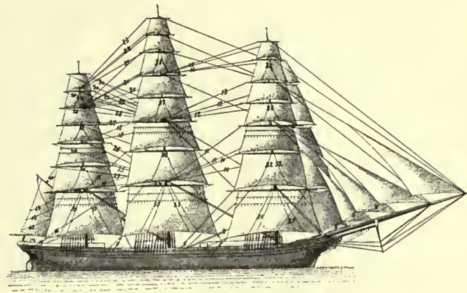
Fig. 122. Ship—Running Rigging
