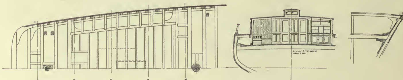
Sections of Auxiliary Schooner, Building From Alden Designs
