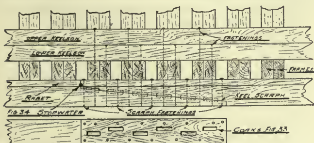
Coaked Keel Scarph and Stopwater
