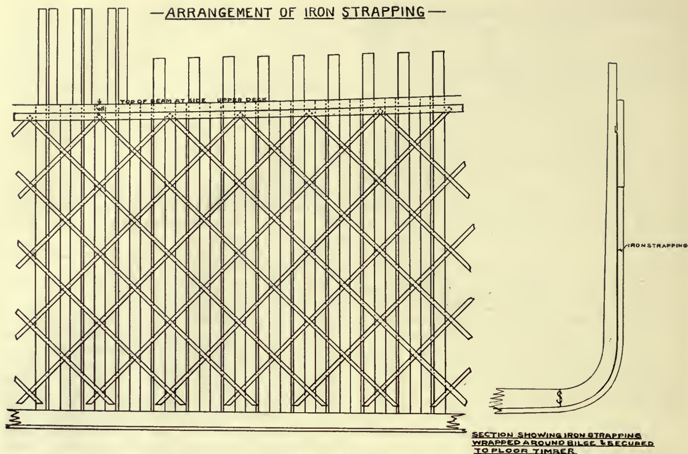
Fig. 49. Diagonal Straps
