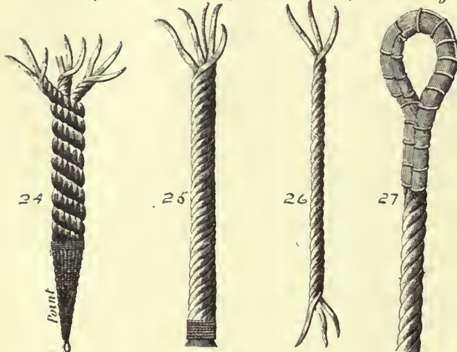
Cable laid Rope Shroud laid Rope Bawser laid Rope Flemish Eye
