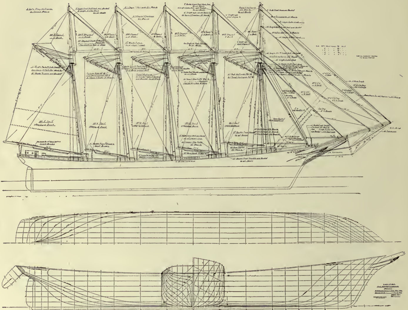
Fig. 200. Lines and Sail Plan of Commercial Schooner. Designed by B. B. Crowninshield
